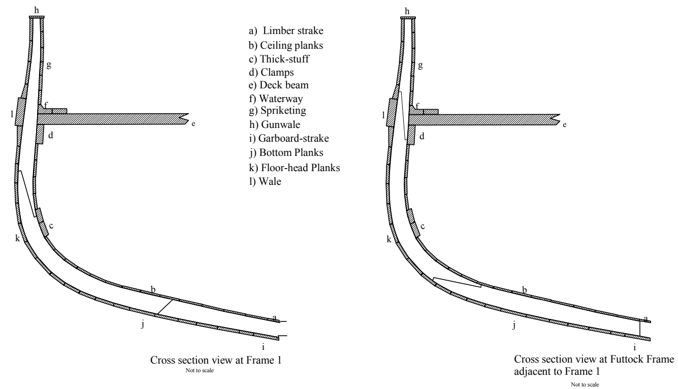
Cross section view at Frame 1
