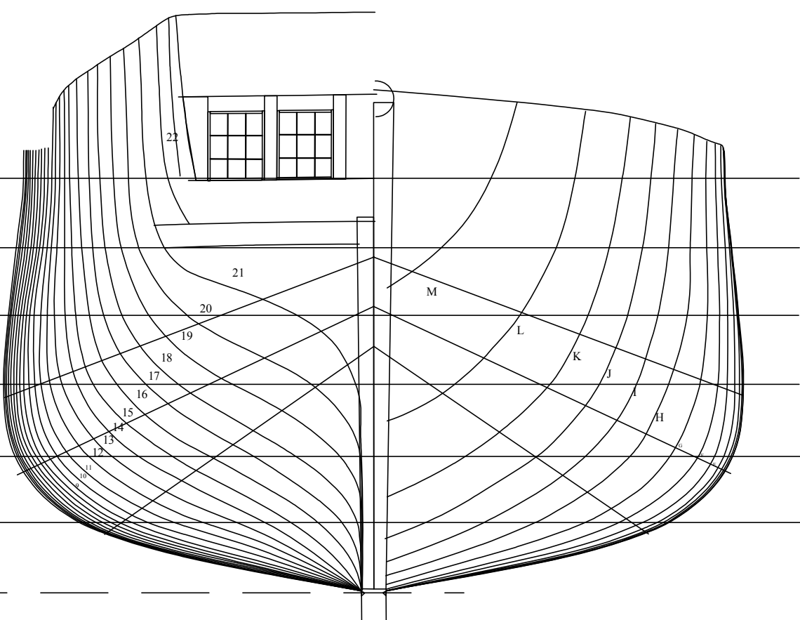
Body Plan
